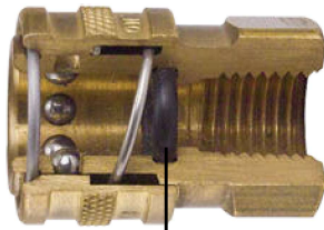
Seal Material
